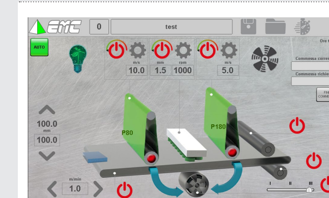
Touch screen 7" - 10" Touch screen 7" - 10" 7-10-Zoll-Touchscreen
